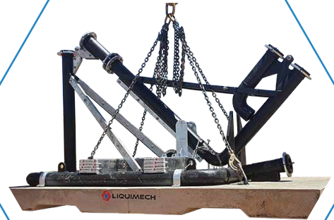
Engineered Concrete Tie Down Blocks for Cyclonic Regions
